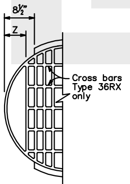
CROSS BAR DETAIL (WELDED STEEL)
