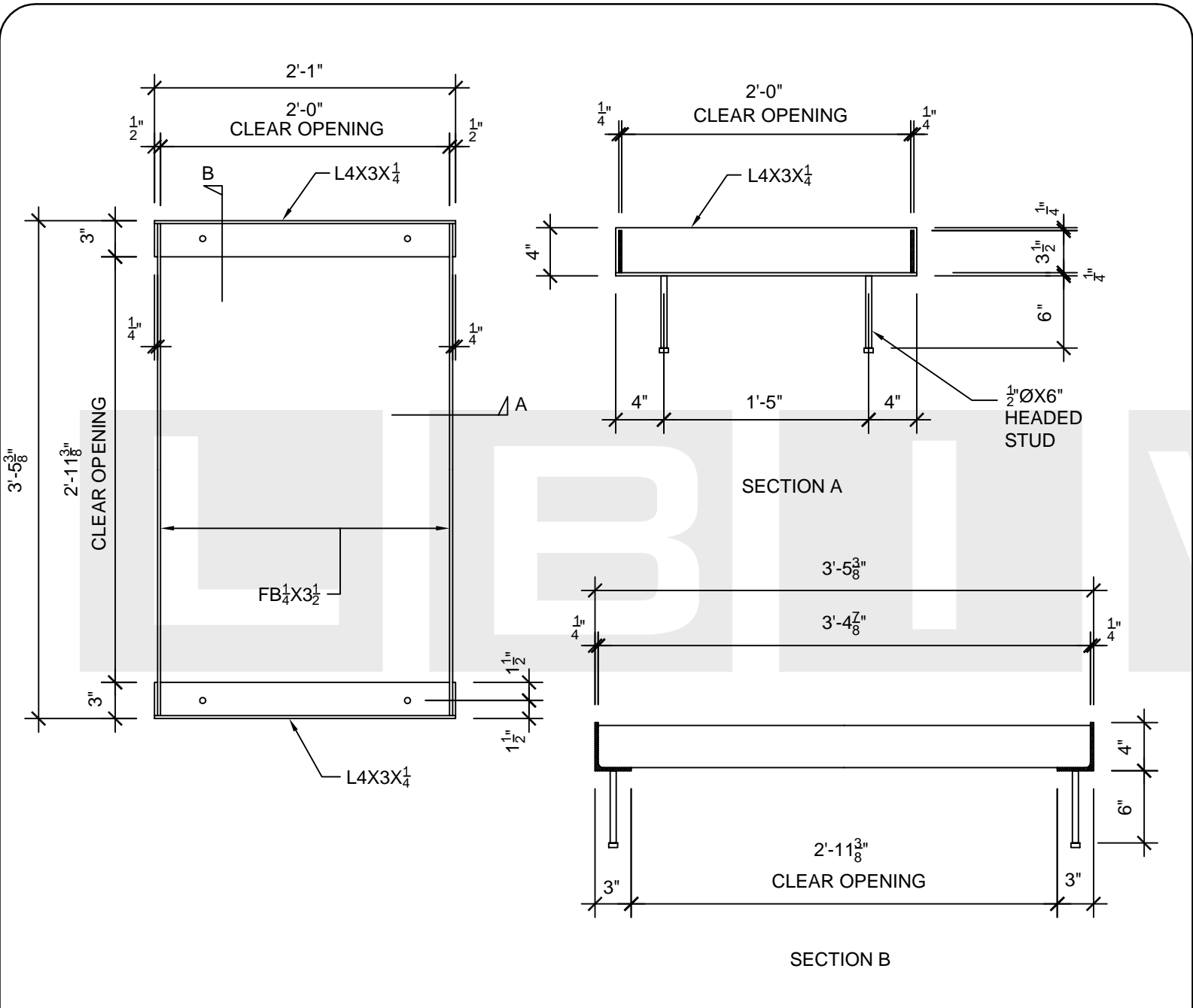
TYPE 24 FRAME DETAILS (For all Rectangular Grates)
