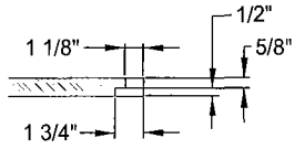
PICK HOLE DETAIL
