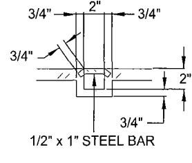
SECTION D-D HANDLE SLOT DETAIL
