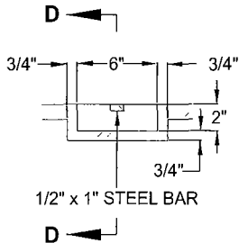
SECTION C-C HANDLE SLOT DETAIL
