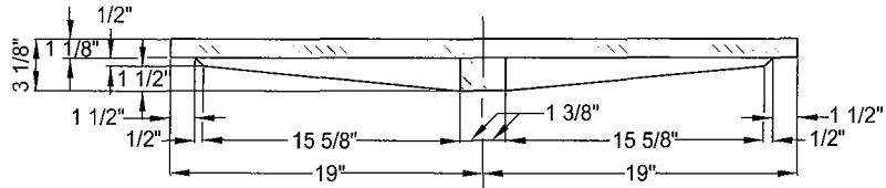
SECTION B-B, COVER B
