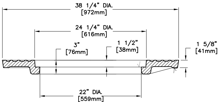
SECTION OF COVER
