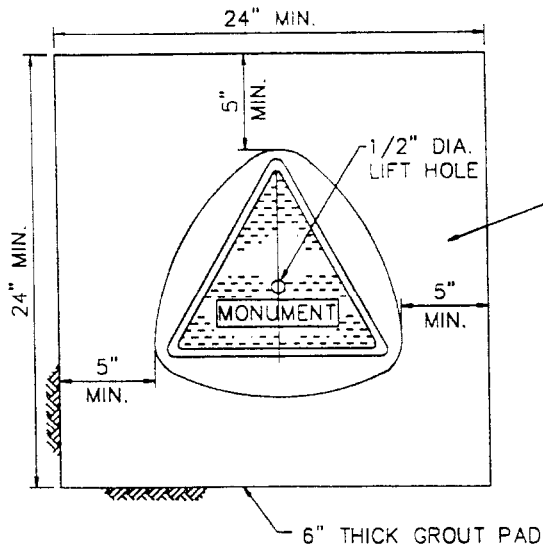
PLAN-IN UNPAVED AREA
