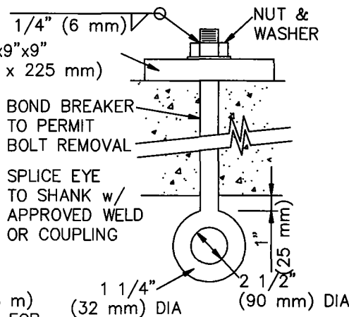
DETAIL J
