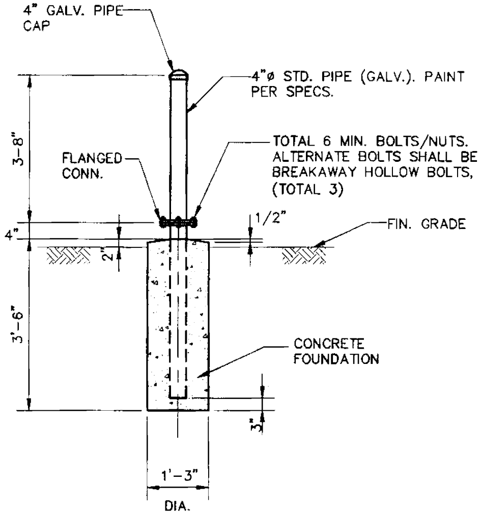
BREAKAWAY GUARD POST DETAIL
