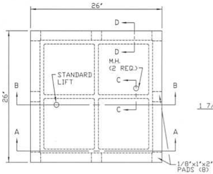
MANHOLE COVER
