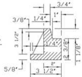
SECTION E-E
