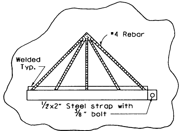
GRATE ASSEMBLY DETAIL
