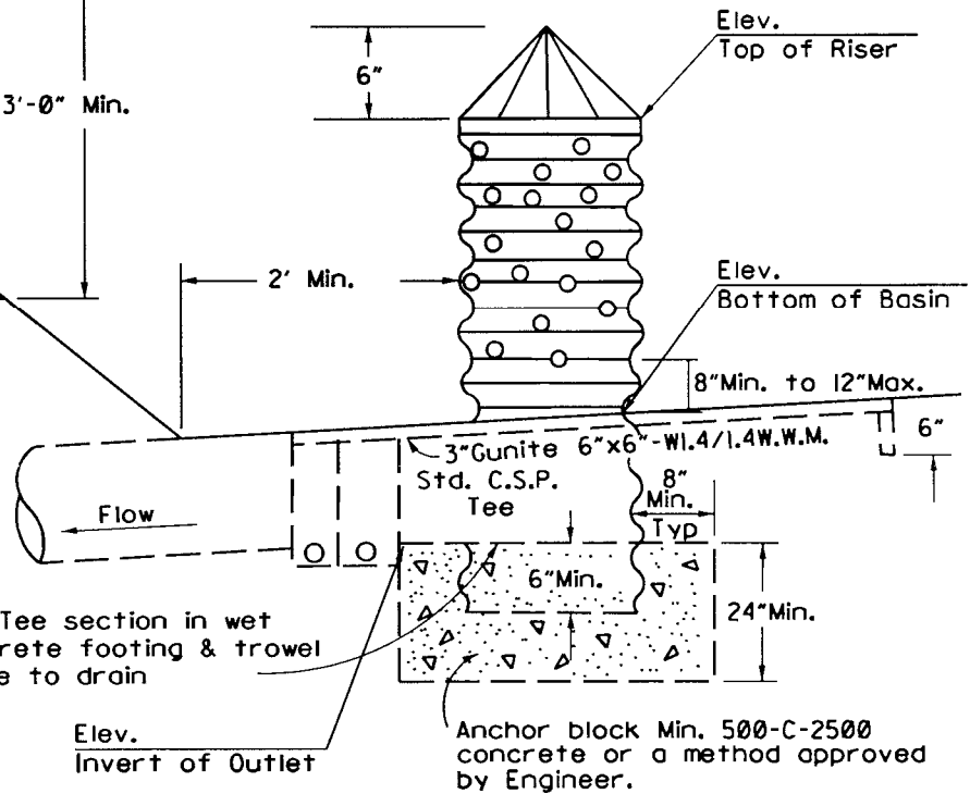
DRAIN PIPE & RISER
