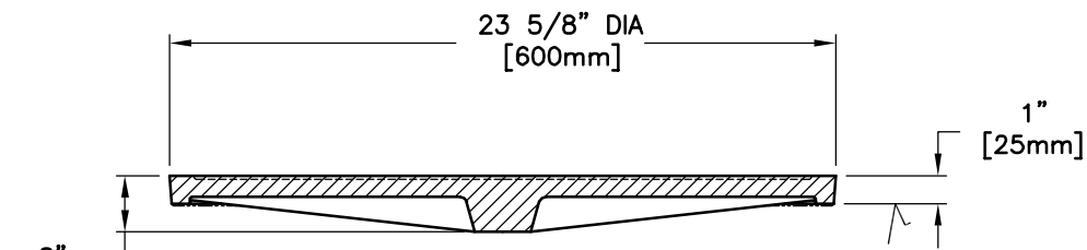
COVER SECTION
