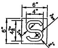
PLAN OF LETTER FOR SEWER COVER
