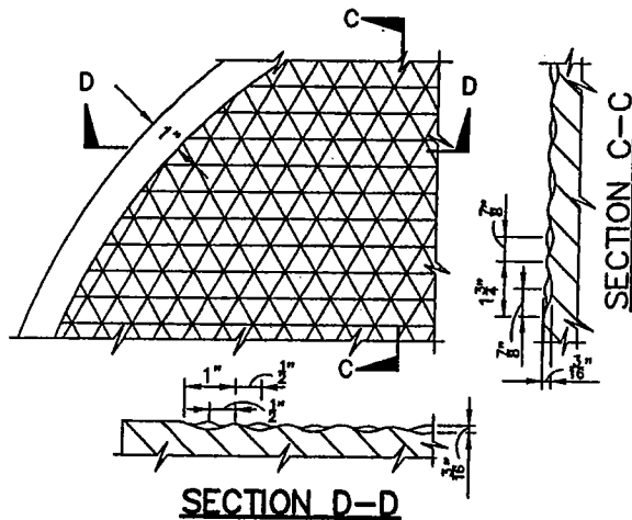
PLAN OF BOTTOM
