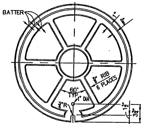
PLAN OF BOTTOM
