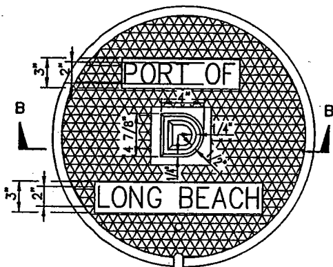
PLAN OF TOP FOR STORM DRAIN COVER
