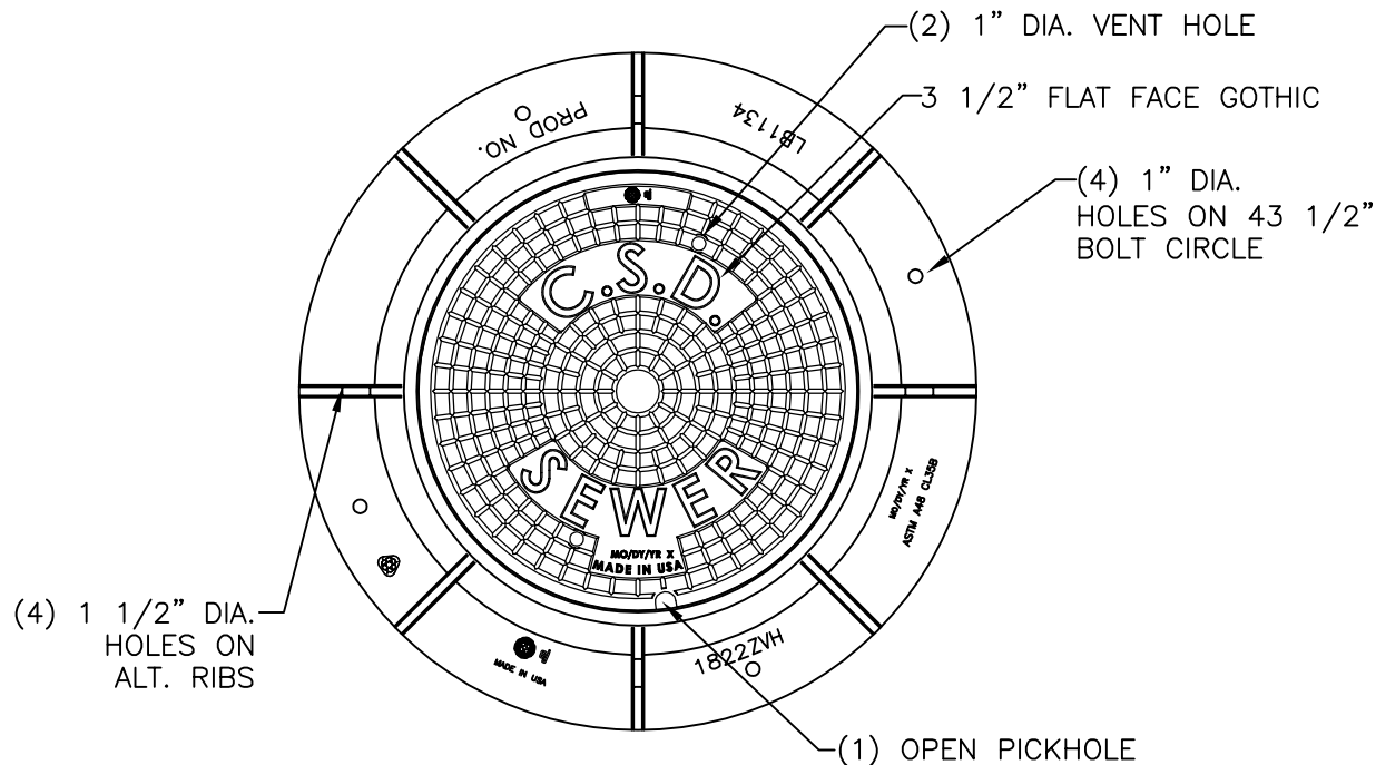
PLAN VIEW
