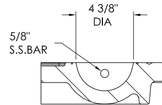
PICKBAR DETAIL
