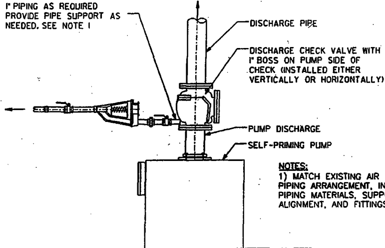
SELF-PRIMING PUMP AIR RELEASE VALVE SYSTEM DETAIL
