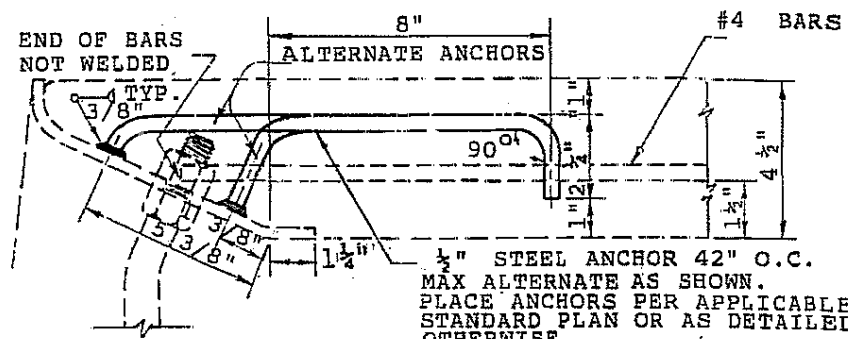
TYPE "B" FACE PLATE ANCHORS
