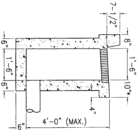
TYPE 2 CURB
