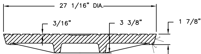
COVER SECTION
