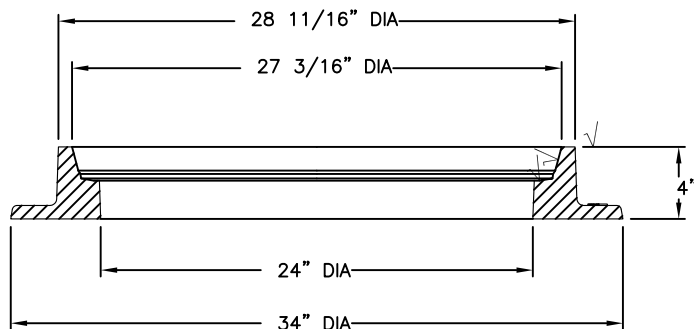
FRAME SECTION
