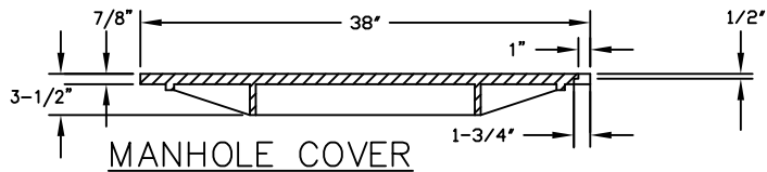
MANHOLE COVER
