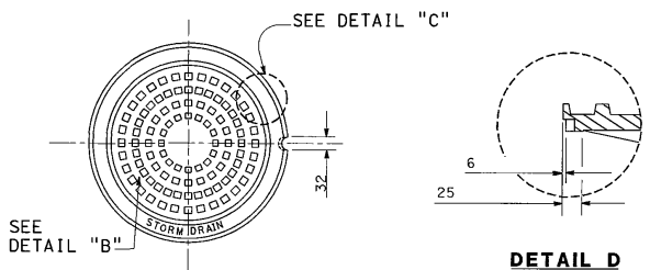
DETAIL D
