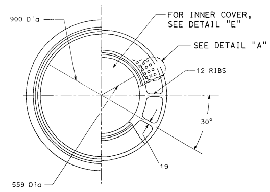
HALF PLAN FRAME AND COVER
