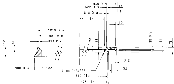
HALF SECTION FRAME AND COVER
