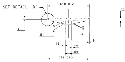
900 mm MANHOLE FRAME AND TWO CONCENTRIC COVERS HEAVY DUTY
