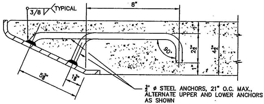
HOOK ANCHOR
