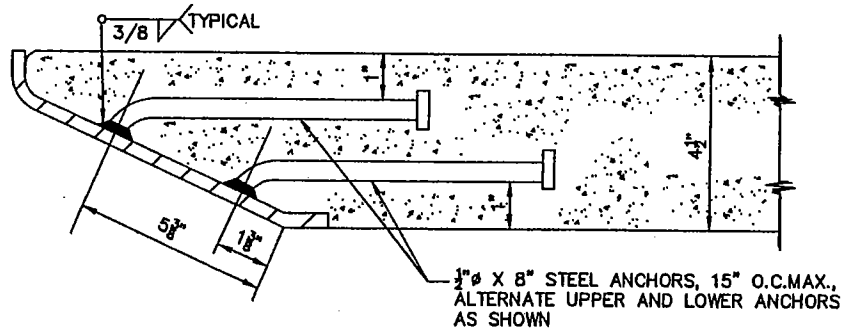
ROUND HEAD ANCHOR
