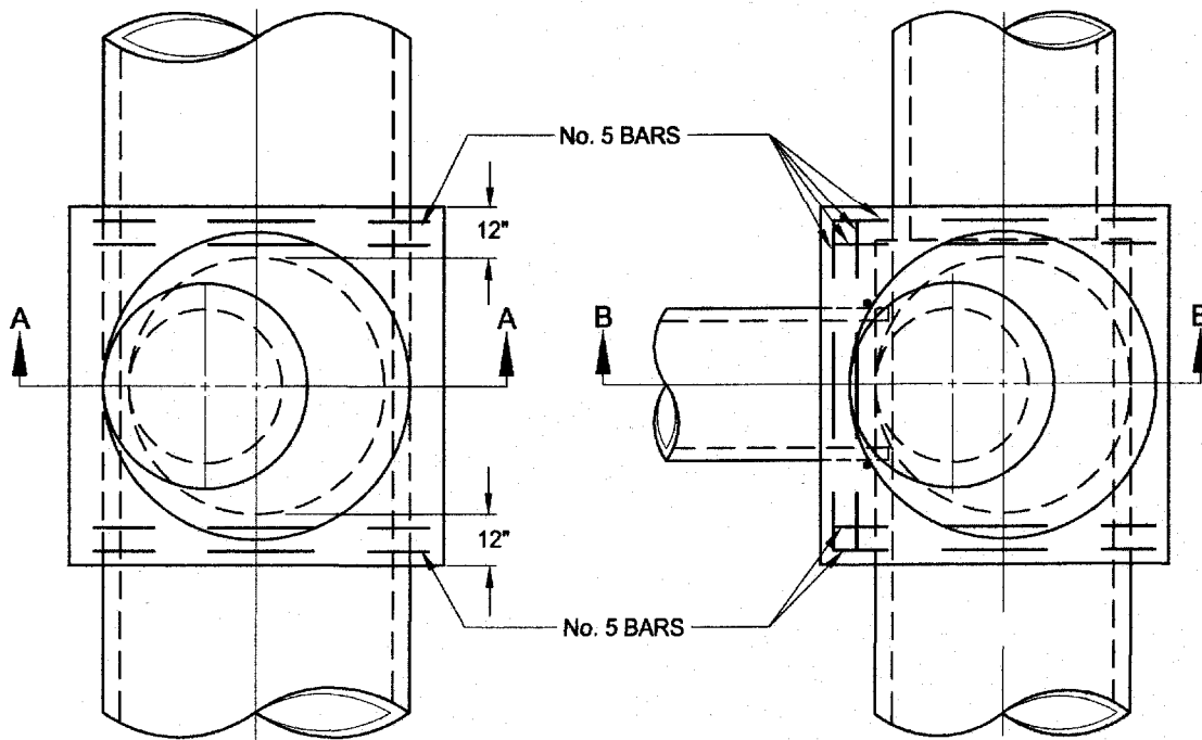
PLAN THROUGH MANHOLE
