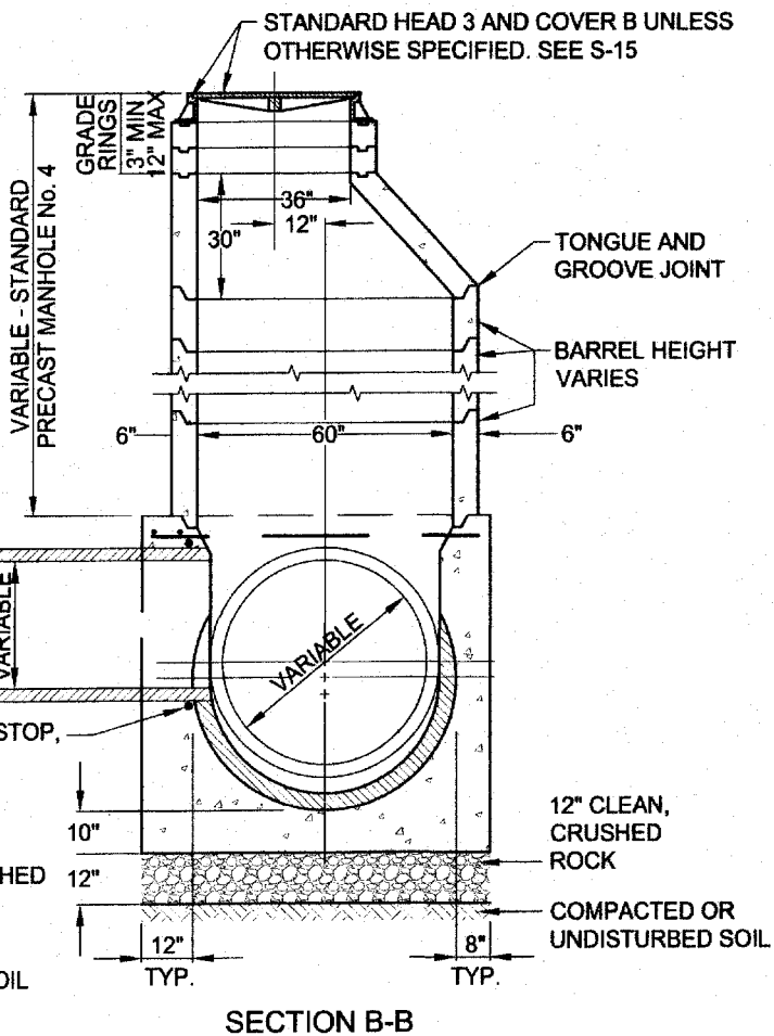
SECTION B-B
