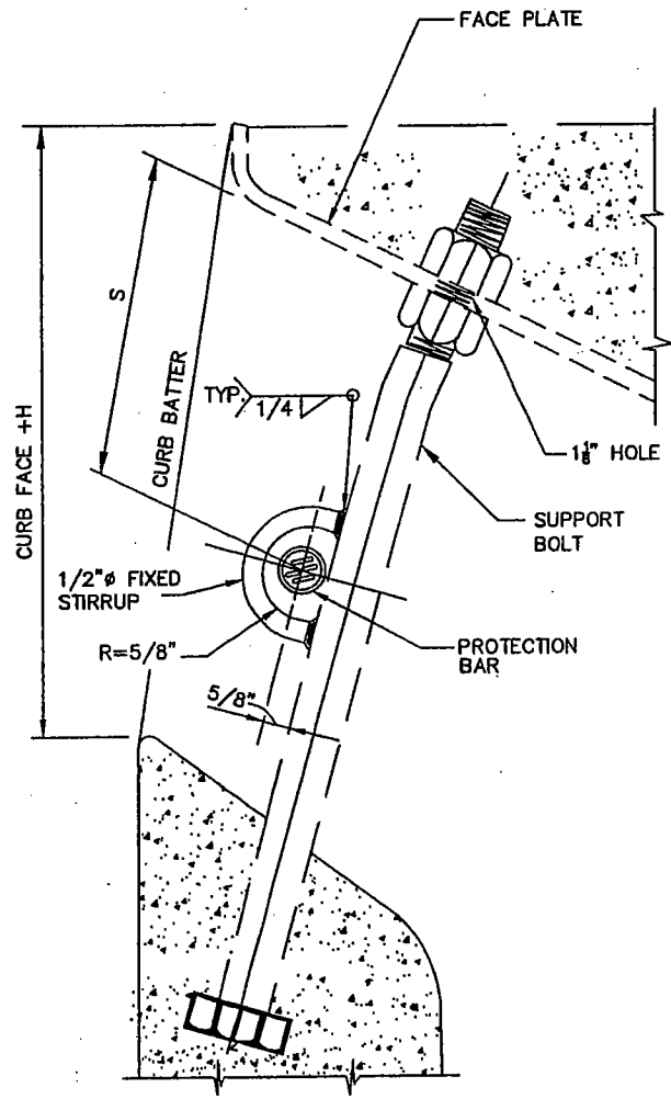
STIRRUP DETAIL
