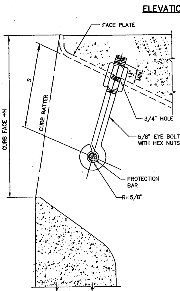
EYE BOLT DETAIL
