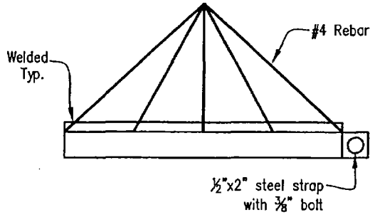
GRATE ASSEMBLY DETAIL
