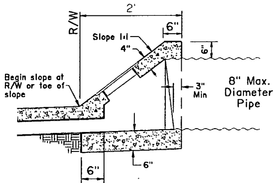
CASE I INLET Pipe
