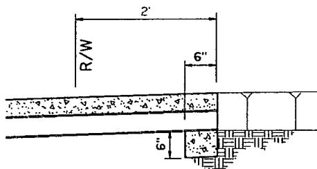
CASE II INLET Open Ditch
