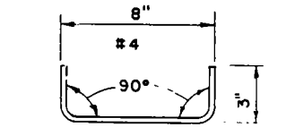
DOWEL DETAIL
