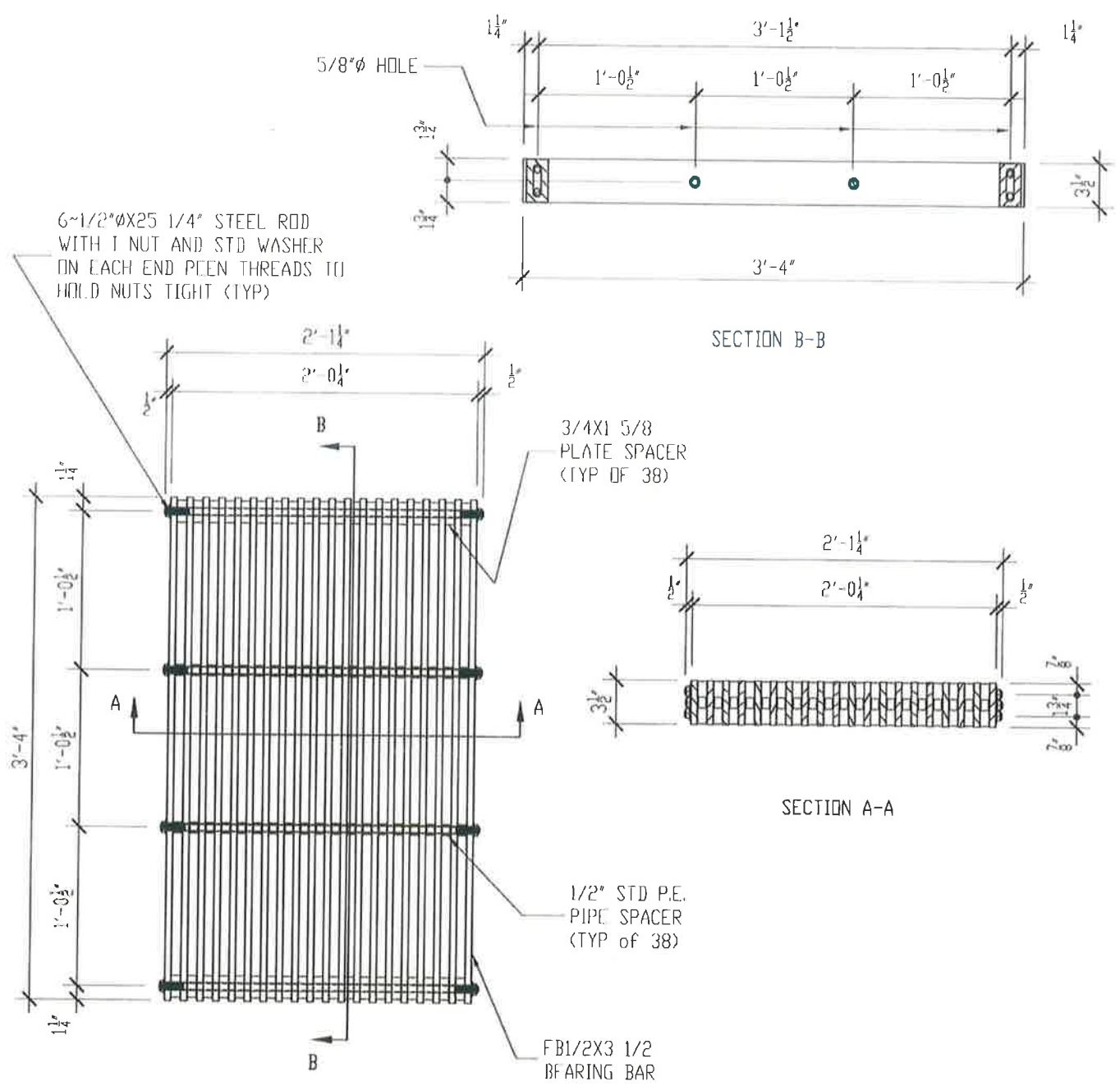
LB 319 RECTANGULAR GRATE ASSEMBLY
