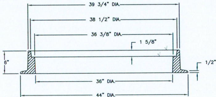
FRAME SECTION
