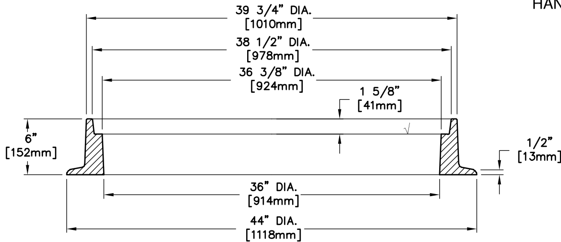
FRAME SECTION
