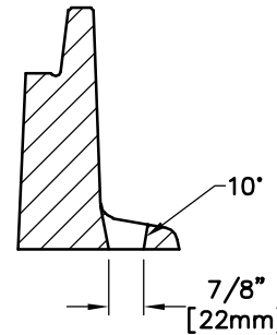
HANDLING HOLE DETAIL
