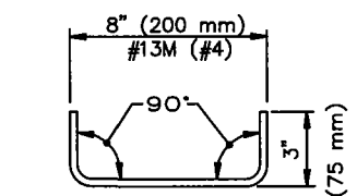
DOWEL DETAIL
