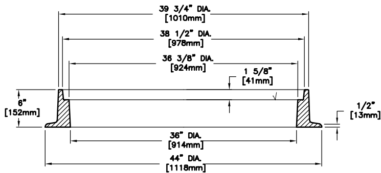
FRAME SECTION
