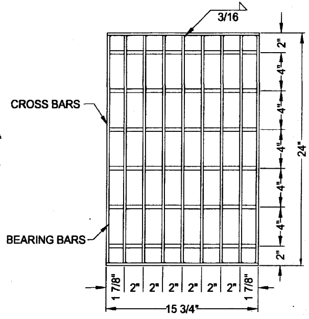
GRATE PLAN
